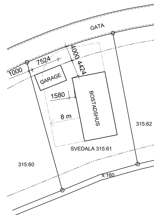
SITUATIONSPLAN 1:500
